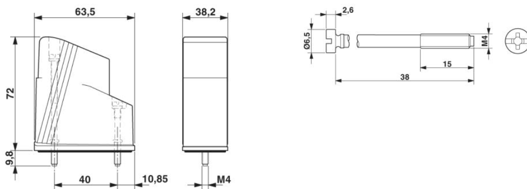
Dimensioned drawing
