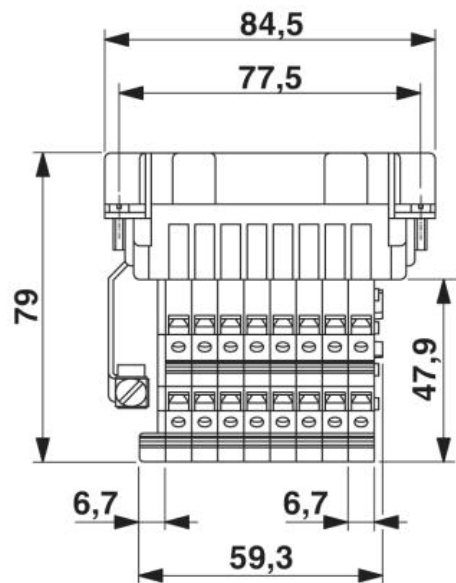
Dimensioned drawing
