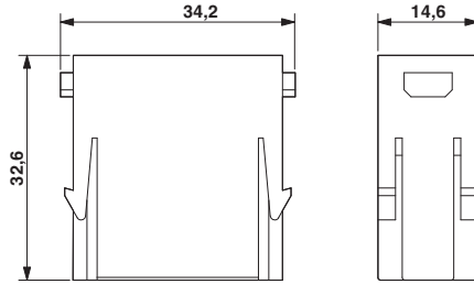
Male insert
