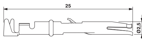
Dimensioned drawing
