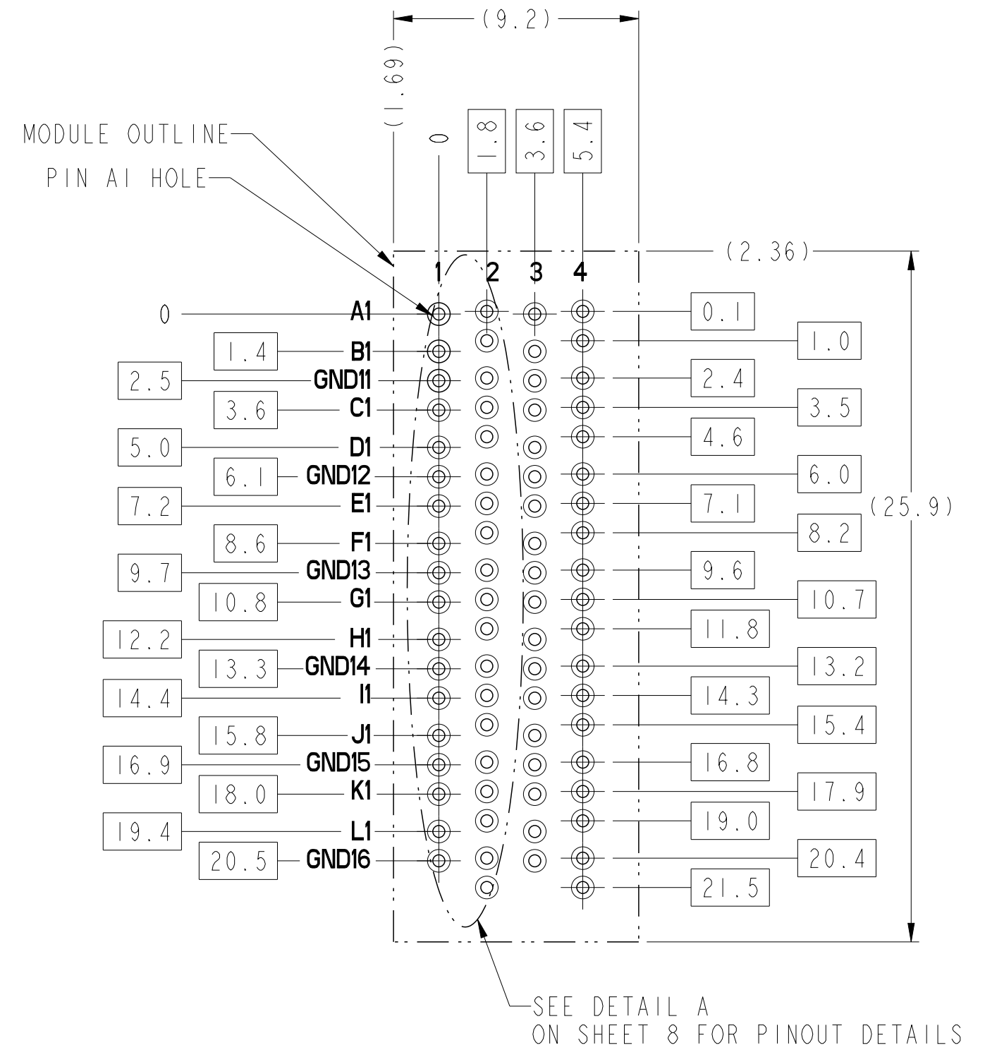
FOUR WALL MODULE BACKPLANE FOOTPRINT
