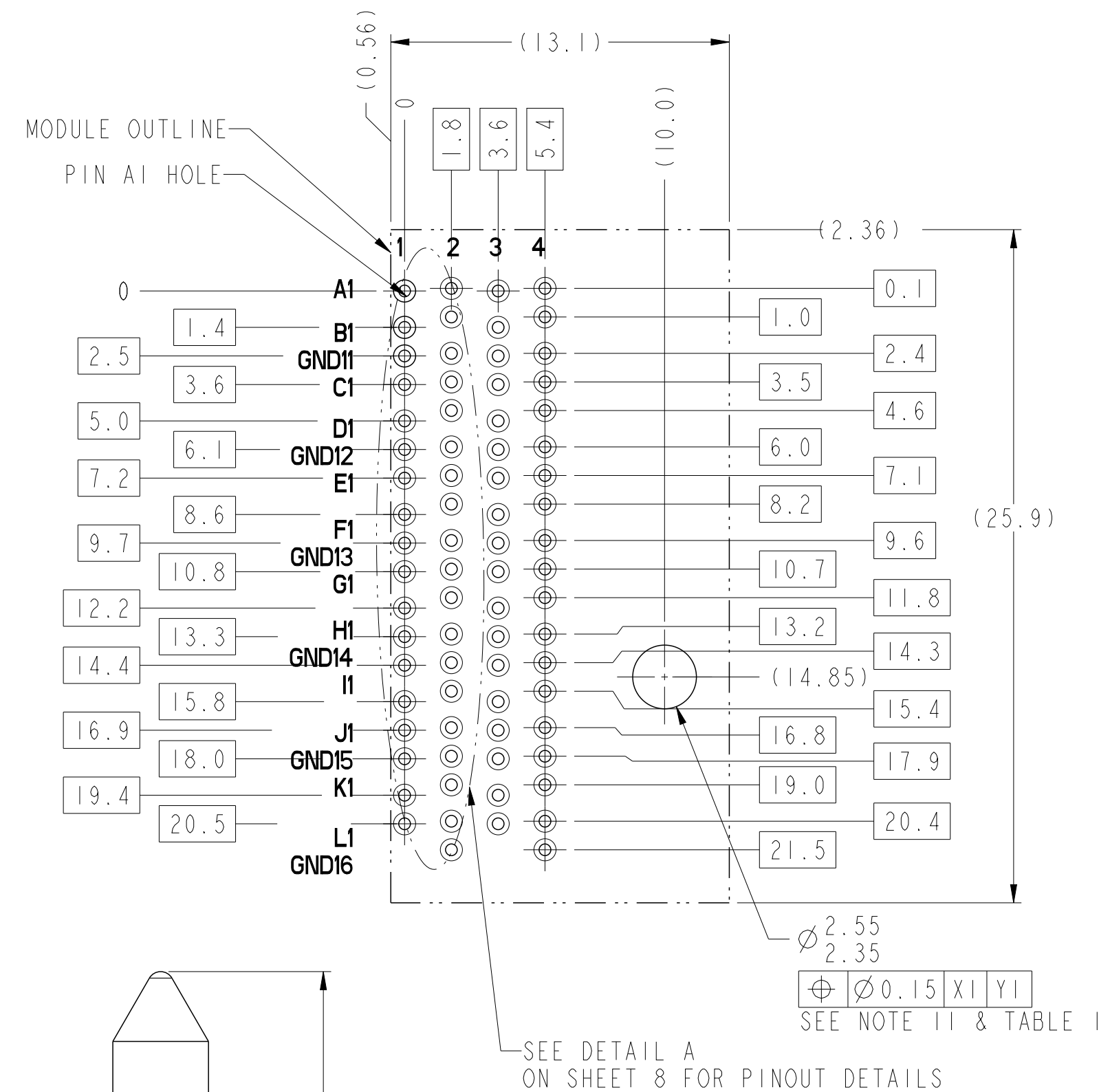
BP HOLE PATTERN COMPONENT SIDE RIGHT POLARIZING GUIDE MODULE BACKPLANE FOOTPRINT
