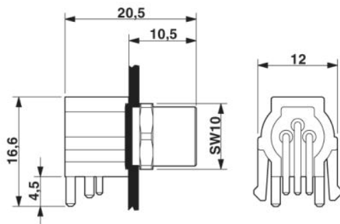
M8 flush-type plug
