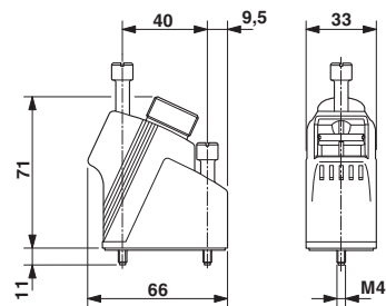
Dimensioned drawing
