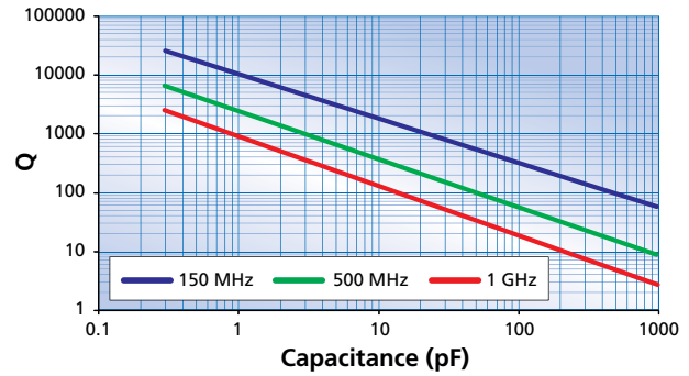
Q vs Capacitance 1111 case size
