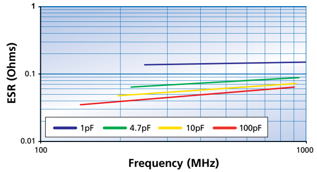
ESR vs Frequency 1111 case size
