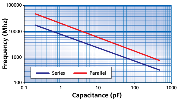
Resonant Frequency vs Capacitance 0805 case size
