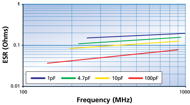
ESR vs Frequency 0805 case size
