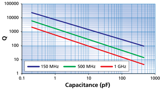
Q vs Capacitance 0805 case size
