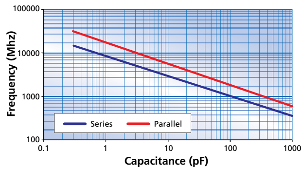
Resonant Frequency vs Capacitance 1111 case size
