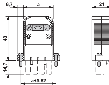
Dimensional drawing
