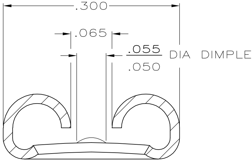
SECTION X-X SCALE 10:1
