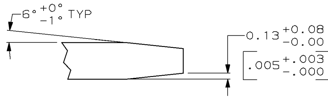
DETAIL X SCALE 20:1
