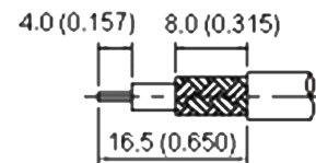
Stripping Dimension
