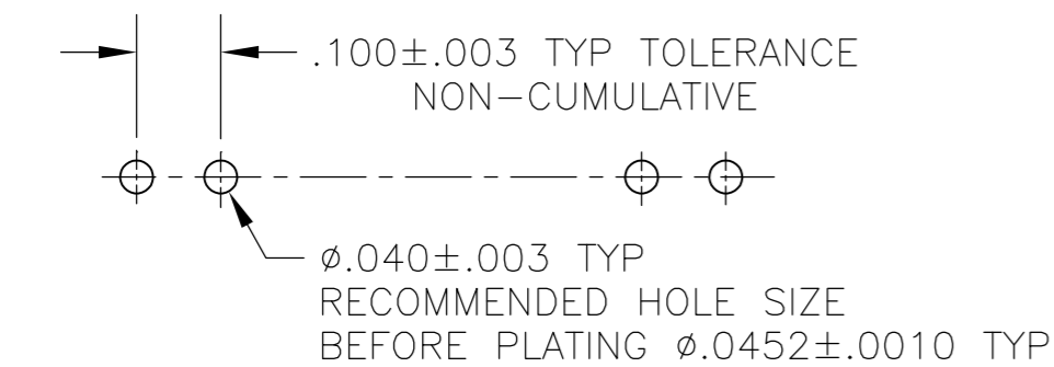
RECOMMENDED HOLE LAYOUT
