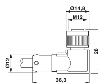
Dimensioned drawing
