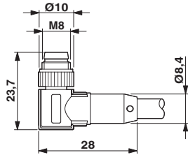
M8 x 1 male plug, angled version
