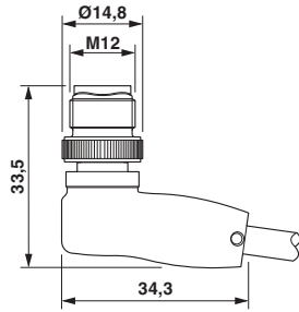
Dimensioned drawing
