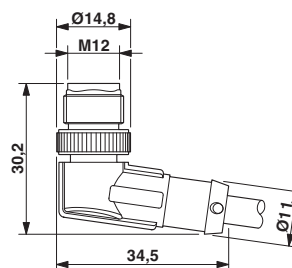
Dimensioned drawing
