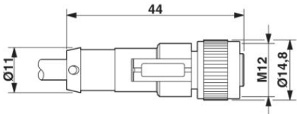
M12 x 1 female connector, straight
