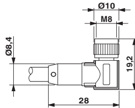
Dimensioned drawing
