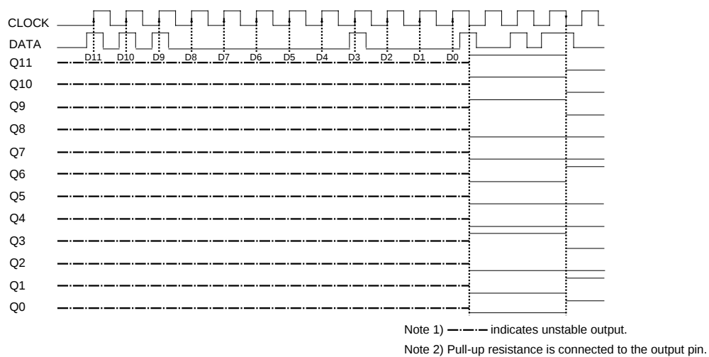
Fig.3 Operation timing chart
