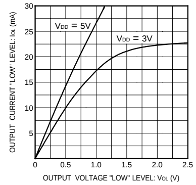
Fig.9 Output current vs. output low level voltage
