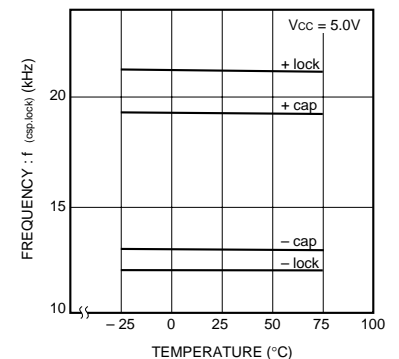
Fig. 19 Capture range charging / lock range vs. temperature
