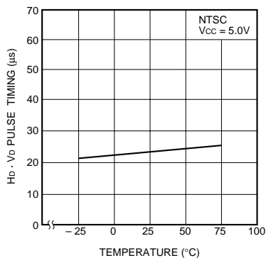
Fig. 17 H D , V D phase difference vs. temperature
