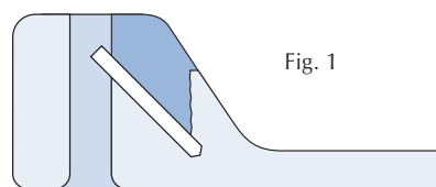
Steel locking barb anchored in tie head
