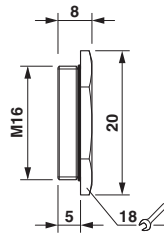
Dimensional drawing
