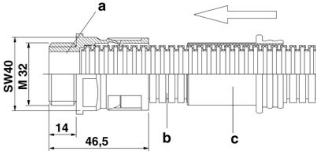
Dimensioned drawing
