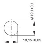
Drilling diagram
