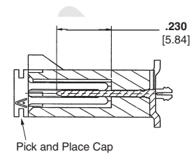
Section K-K
