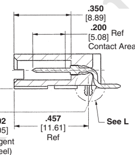
Section K-K
