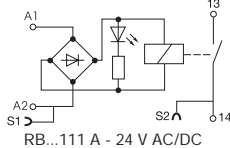
RB...111 A - 24 V AC/DC
