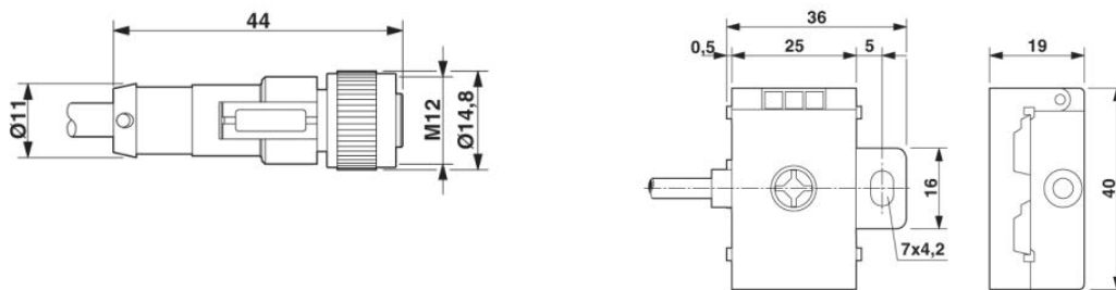
Dimensioned drawing
