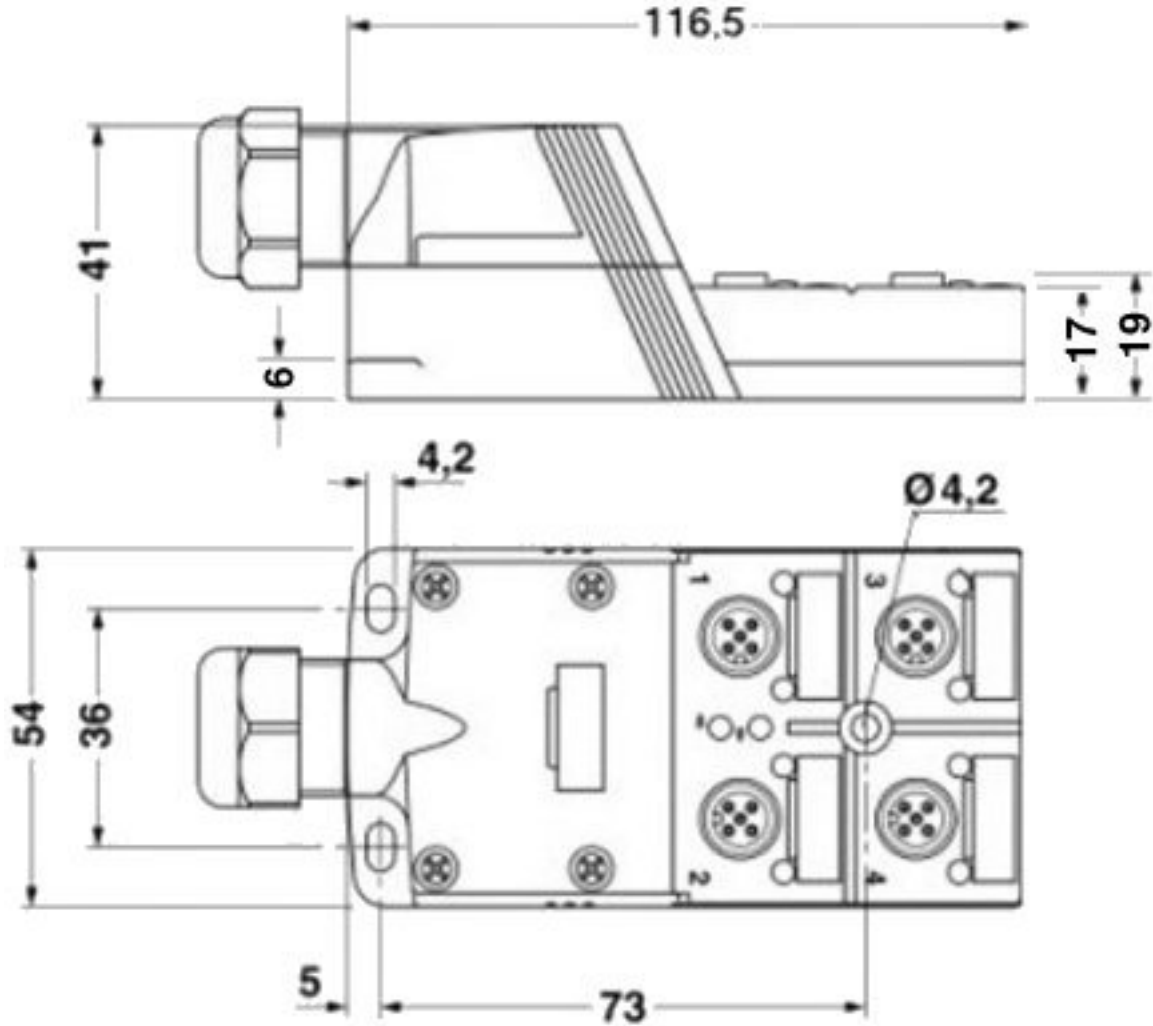
Dimensional drawing
