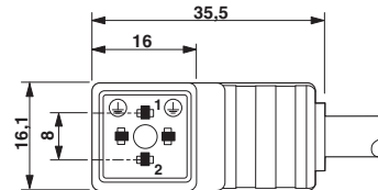
Dimensioned drawing
