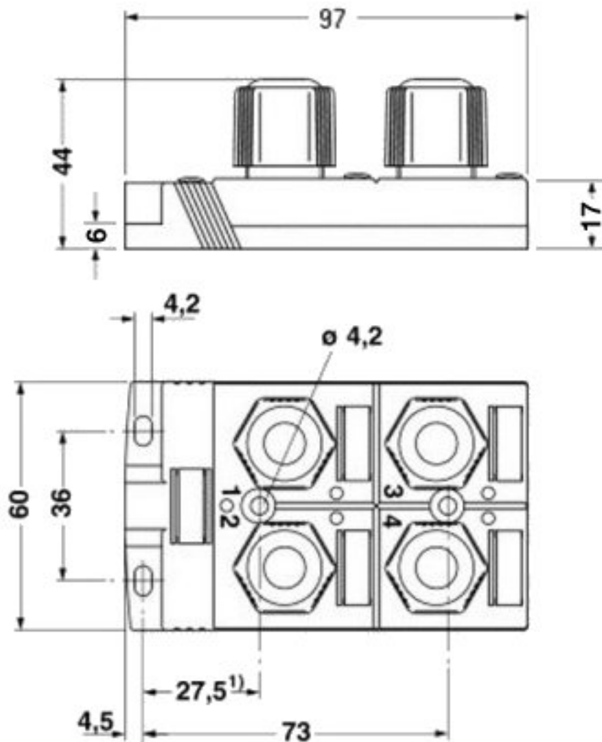
Dimensioned drawing
