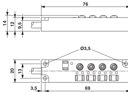
Dimensioned drawing
