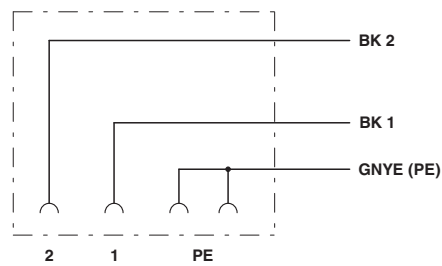
Circuit diagram
