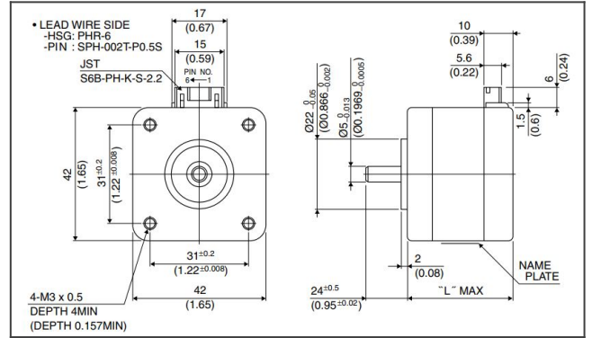
17pmk product drawing
