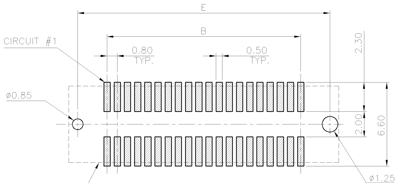
RECOMMENDED P.C.B. LAYOUT (TOLERANCE: ±0.05)
