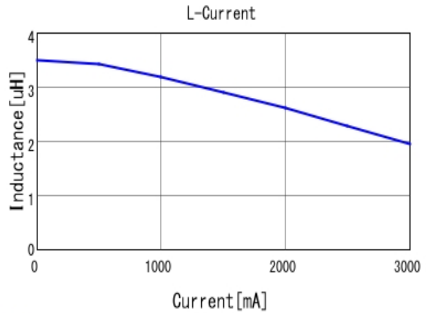
■ 1276AS-H-3R3M L-Current 20degC
