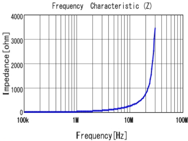
■ 1276AS-H-3R3M |Z|
