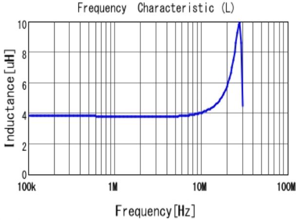
■ 1276AS-H-3R3M L
