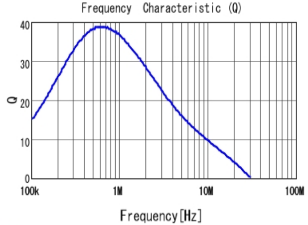
■ 1276AS-H-3R3M Q
