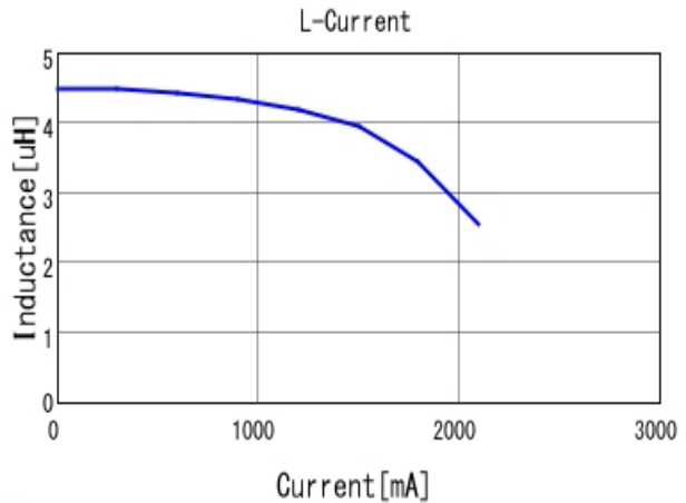
■ 1231AS-H-4R7M L-Current 20degC
