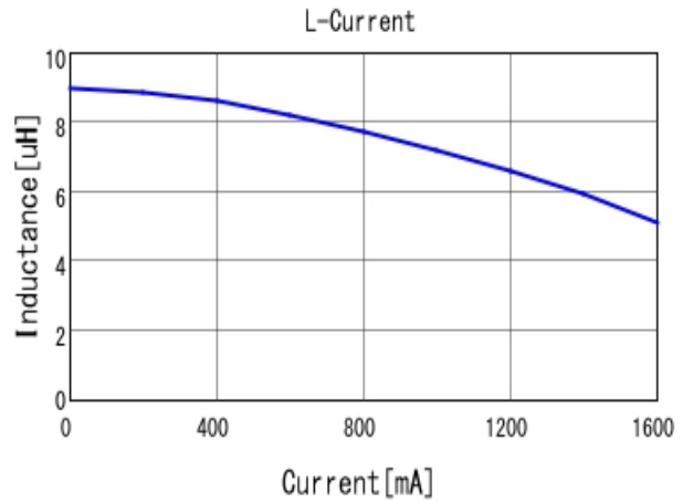
■ 1269AS-H-100N L-Current 20degC
