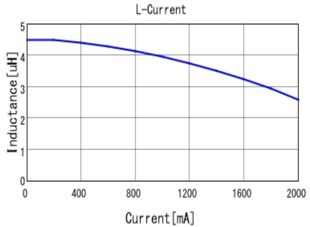
■ 1269AS-H-4R7M L-Current 20degC
