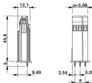
Dimensioned drawing
