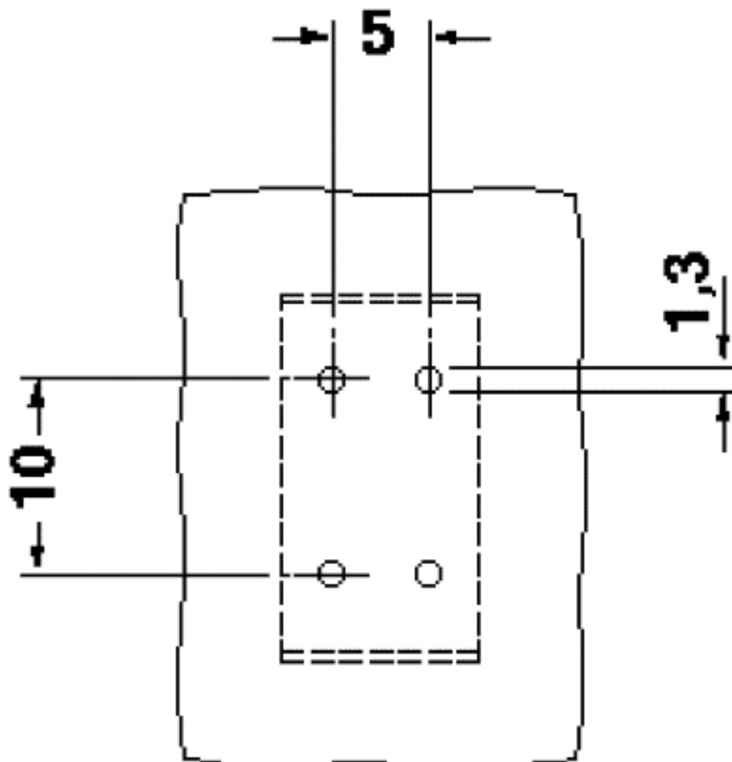
Drilling diagram
