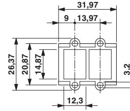
RJ45 panel mounting frame, IP20
