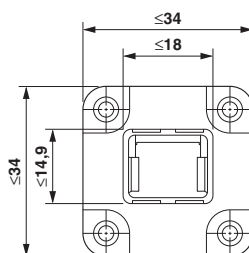
Dimensioned drawing
