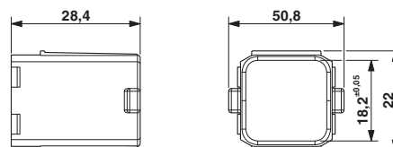
Dimensioned drawing
