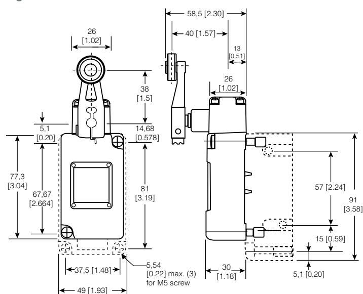
Figure 34. 201LS3-4 Dimensions
