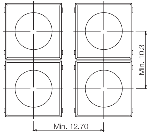
through-hole
