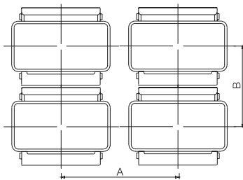
Switch spacing
