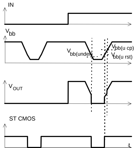
Figure 6a: Undervoltage:
