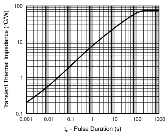
Fig. 12 - Typical Transient Thermal Impedance
