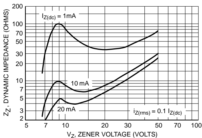
Figure 4. Effect of Zener Voltage
