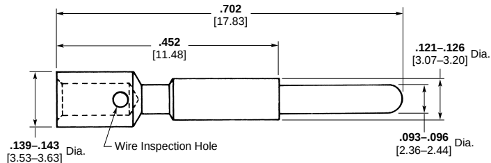
Part Number 083-0173-00R4 12 AWG Pin
