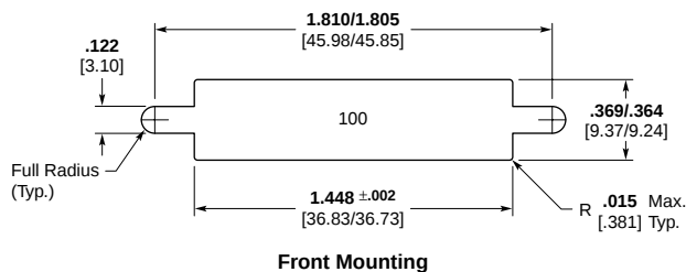
Front Mounting
