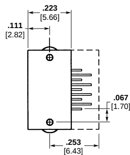
Horizontal Surface Mount
