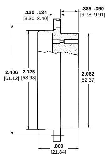
Receptacle Part Number 204027-2
