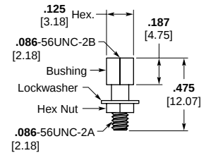
Part Number 5-1532137-9 Jackpost Assembly (P) S96-0002-0009 M83513/5-07 P mates with K, KM, L, LM, Q, QM and R, RM Jackscrew Assemblies.
