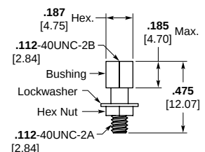
Part Number 6-1532137-4 Jackpost Assembly (S) S96-0002-0060 M83513/5-17 S mates with H, HM, J, JM, T, TM and N, NM Jackscrew Assemblies.
