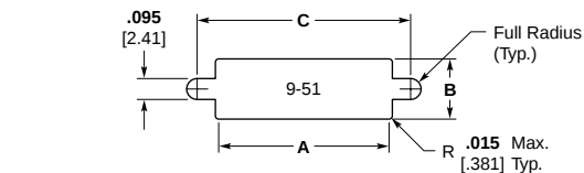
Figure 1 Front Mounting
