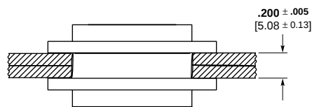
Plug and Receptacle Rear Mounted
