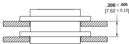
Plug Front Mounted Receptacle Rear Mounted
