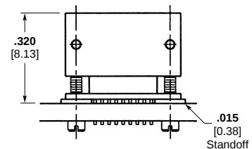
Vertical Thru Hole
